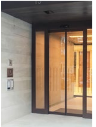
Watertight integrity Leaf with full framed profile, glass up to 30 mm and safety electromagnetic lock.
